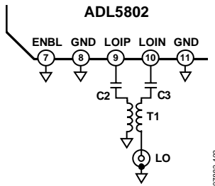
Figure 70. ADL5802 LO Interface
